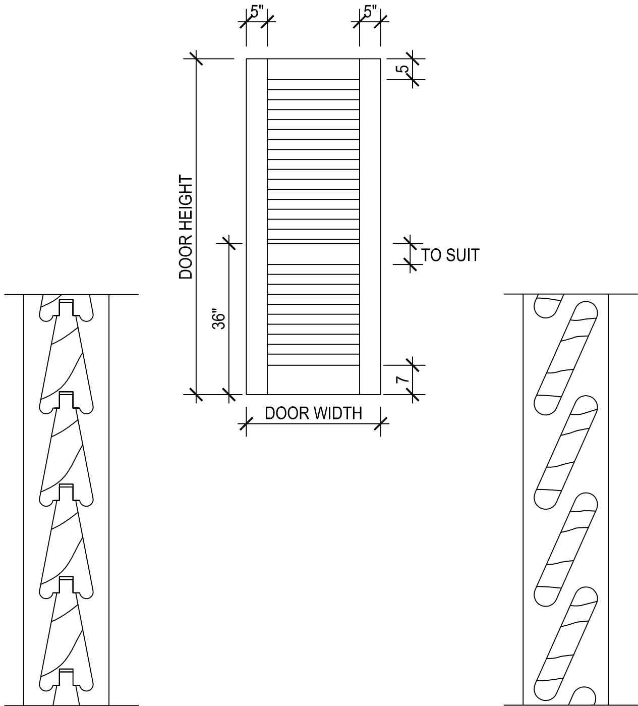
CLOSED LOUVRE
